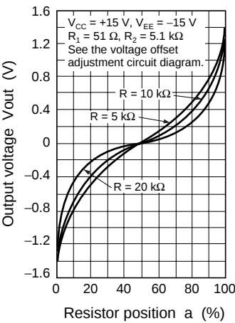
Offset Adjustment Characteristics
