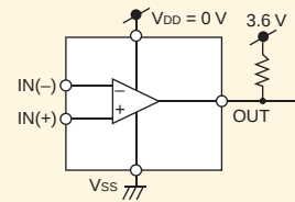
Figure 2: Voltage Application Allowed When V_{DD} = 0 V
