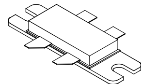
CASE 465M-01 STYLE 1 (NI-780-4)
