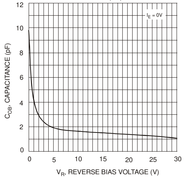
Fig. 4 Output Capacitance
