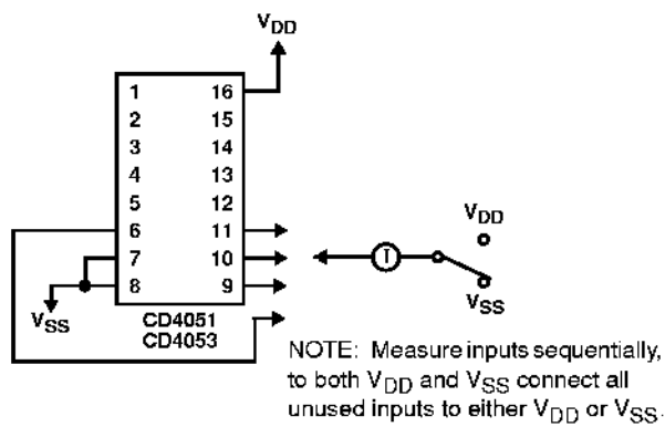
FIGURE 19. INPUT CURRENT
