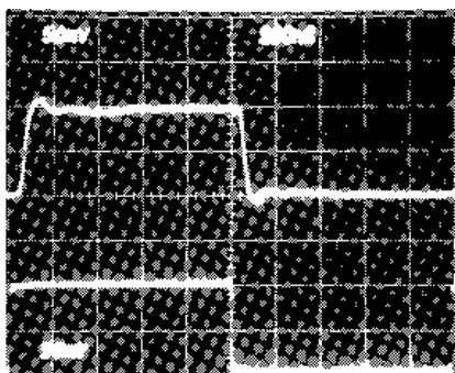
Top Trace: Output; 50mV/Div., 200ns/Div.
