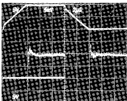
Top Trace: Output Signal; 5V/Div, 2μs/Div.
