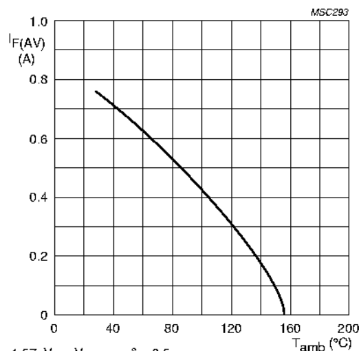
Fig.3 Maximum permissible average forward current as a function of ambient temperature (including losses due to reverse leakage).
