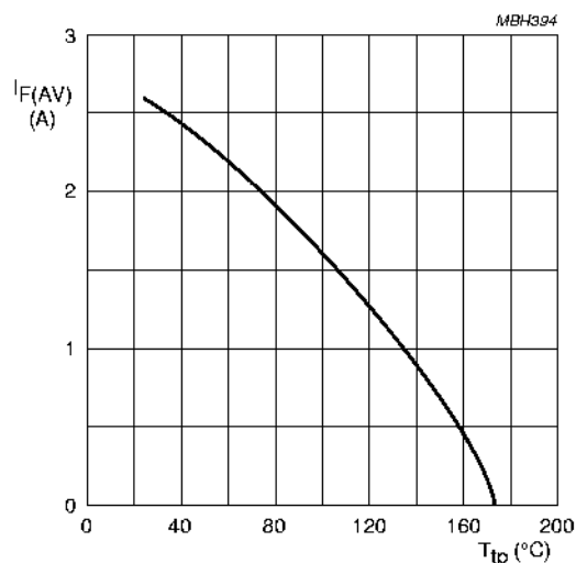
Fig.2 Maximum permissible average forward current as a function of tie-point temperature (including losses due to reverse leakage).
