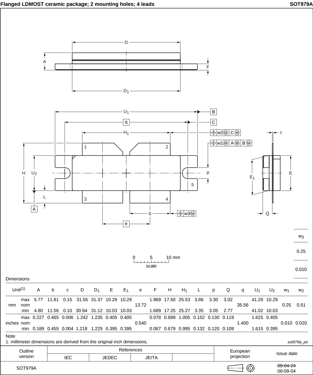
Fig 17. Package outline SOT979A
