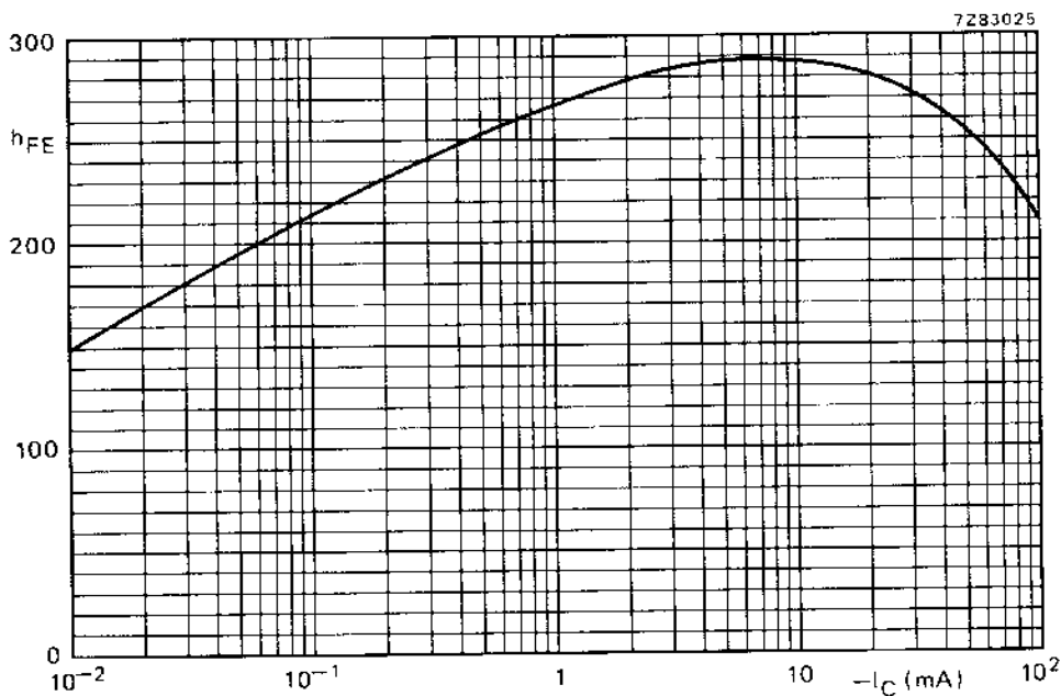
Fig. 4 Typical values of d.c. current gain. -V_{CE} = 5 V; T_j = 25^\circ\text{C} .
