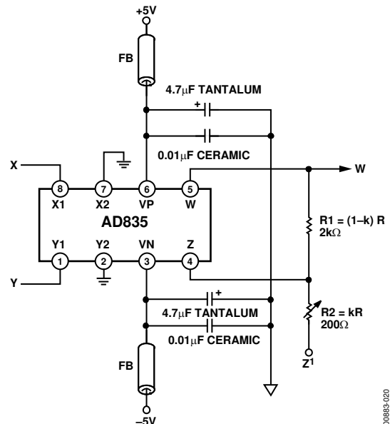
Figure 20. Multiplier Connections
