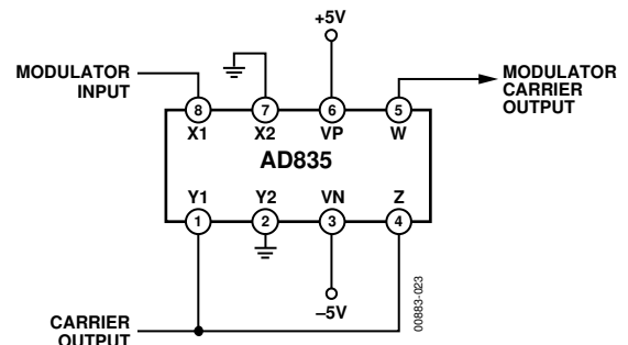
Figure 23. Simple Amplitude Modulator Using the AD835
