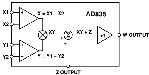
Figure 19. Functional Block Diagram
