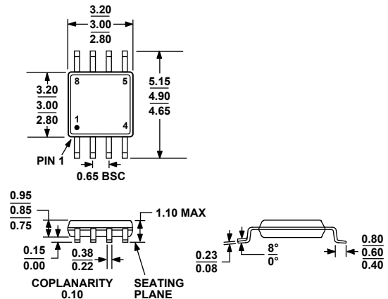
COMPLIANT TO JEDEC STANDARDS MO-187-AA Figure 54. 8-Lead Mini Small Outline Package [MSOP] (RM-8)
