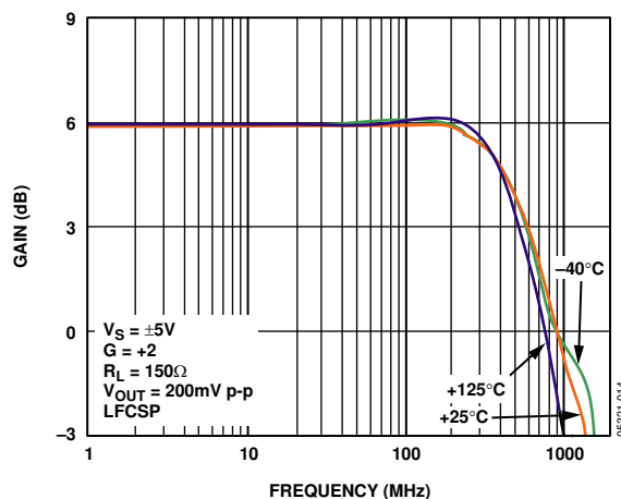
Figure 14. Small Signal Frequency Response vs. Temperature
