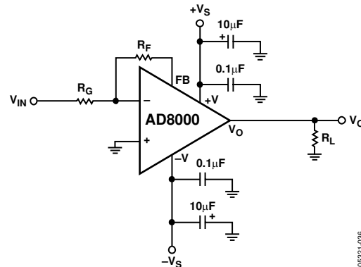
Figure 51. Inverting Configuration
