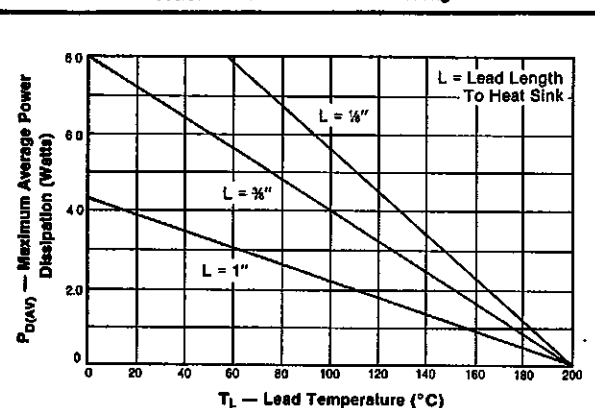
FIGURE 1—Power or Current Derating
